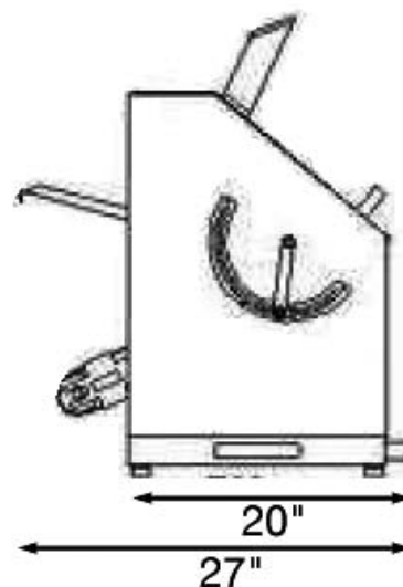
The Unisource Heavy Duty COMPACT BENCH SHEETER™ with 3 Roller, Two Stage Machine for Uniform Dough Sheetting UNI-COMPACT-BDS
